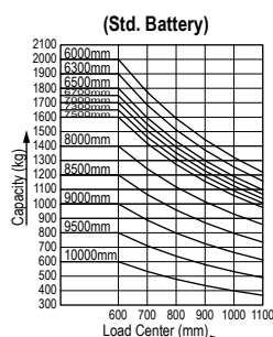
CAPACITY CHART
