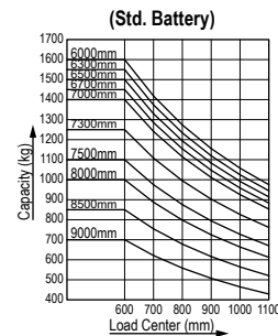
CAPACITY CHART
