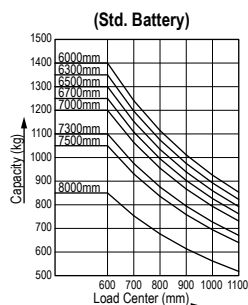
CAPACITY CHART
